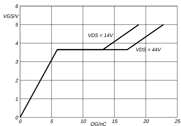
Fig.13. Typical turn-on gate-charge characteristics. V_{GS} = f(Q_G) ; conditions: I_D = 30\text{ A} ; parameter V_{DS}
