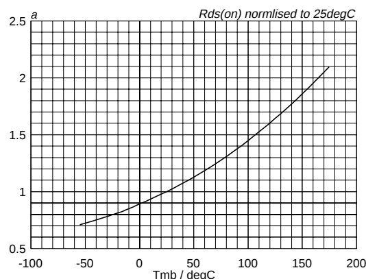
Fig.9. Normalised drain-source on-state resistance. a = R_{DS(ON)}/R_{DS(ON)25^\circ C} = f(T_j) ; I_D = 17\text{ A} ; V_{GS} = 5\text{ V}
