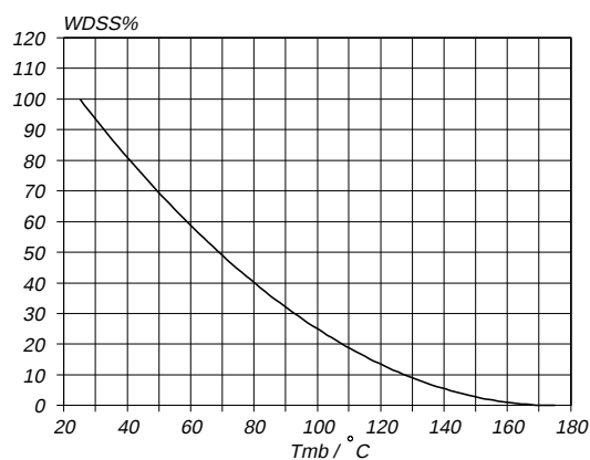
Fig.15. Normalised avalanche energy rating. W_{DSS}\% = f(T_{mb}) ; conditions: I_D = 20\text{ A}
